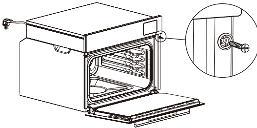
Mounting screw fixing position
