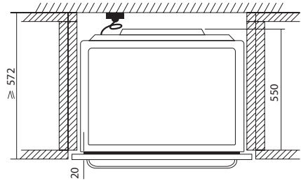
Product top view
