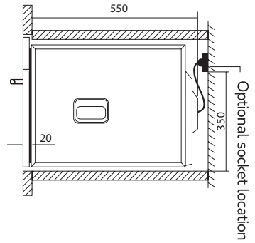
Installation side view
